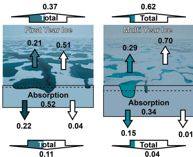
Figure 3. Short-wave albedo, transmittance, and absorption of Arctic first- and multi-year sea ice during summer. Colored arrows refer to melt ponds while white arrows refer to white ice. The pictures show representative photographs of first- and multi-year sea ice. The dashed lines in the sea ice indicate water level. The “Total” arrows average transmittance and albedo over each sea-ice type, considering 23 and 42% ponded surface fractions of multi- and first-year ice, respectively. This fraction is indicated through the colors in the arrows. Albedo for different ice types is taken from Perovich [1996]. Absorption is given in the ice as the sum of white ice and ponds.
