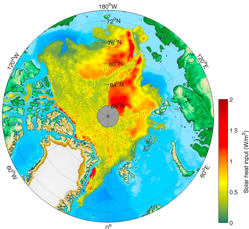
Figure 4. Solar heat input into the Arctic Ocean through sea ice. This map only considers fluxes through sea ice, excluding fluxes through open water, for August 2011.
